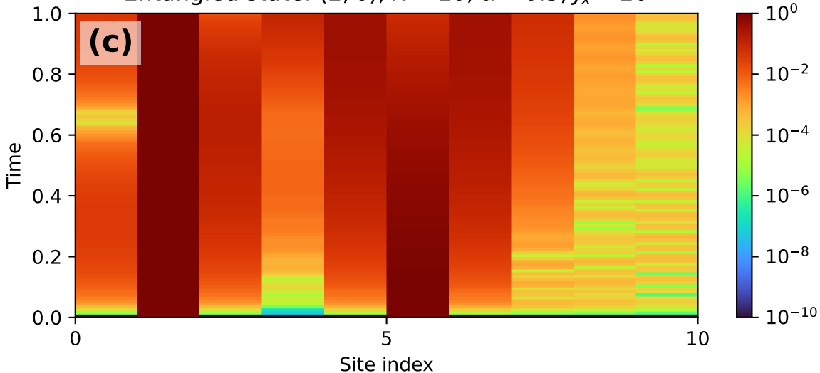
Entangled state: (2; 6) , N = 10 , \alpha = 0.5 , J_x = 20
